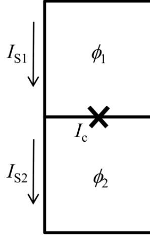
Fig. 18.13. Gradiometer RF SQUID.
