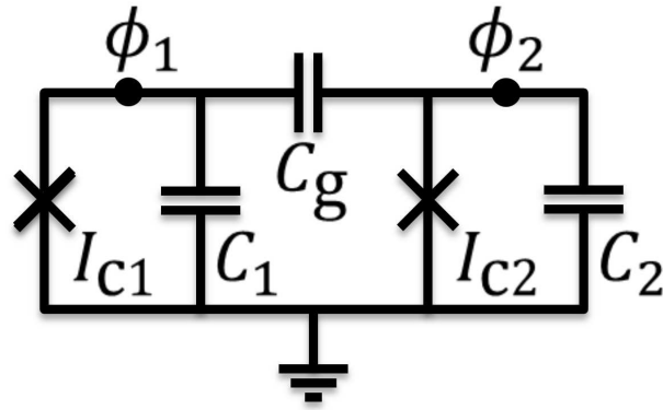
Fig. 18.12. Two coupled charge qubits.
