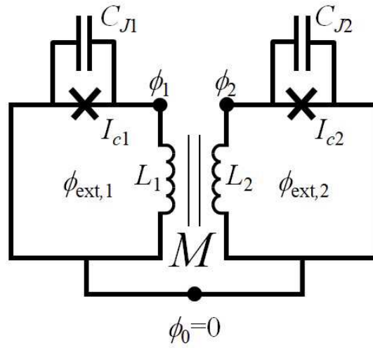
Fig. 18.11. Two coupled flux qubits.
