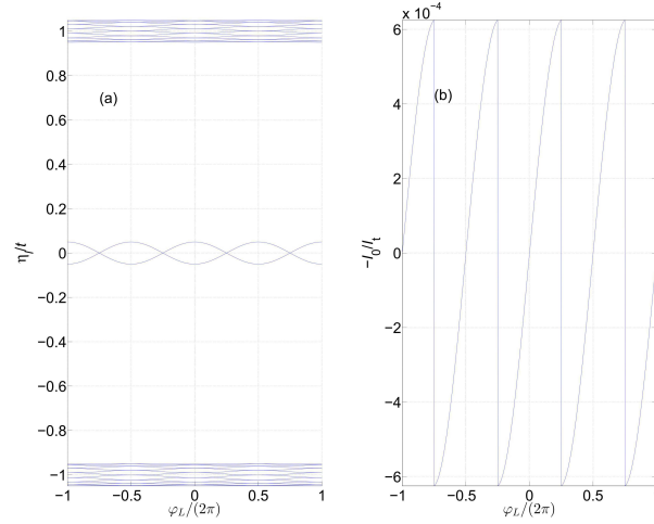
Fig. 18.15. Kitaev RF SQUID. The (a) normalized eigenvalues \{\eta_1/t, \eta_2/t, \dots, \eta_{2L}/t\} of the matrix M (18.981), and (b) normalized ground state current I_0/I_t as a function of \varphi_L [see Eq. (18.1036)].
