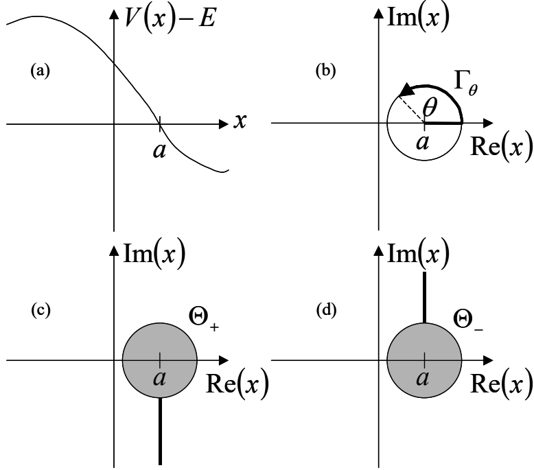
Fig. 11.1. (a) The turning point at x = a . (b) The integration trajectory \Gamma_\theta . The singly connected region \Theta_+ (c) and \Theta_- (d).
