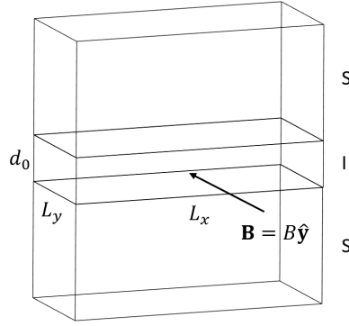
Fig. 18.9. Magnetic field \mathbf{B} = B\hat{\mathbf{y}} applied to a Josephson junction.
